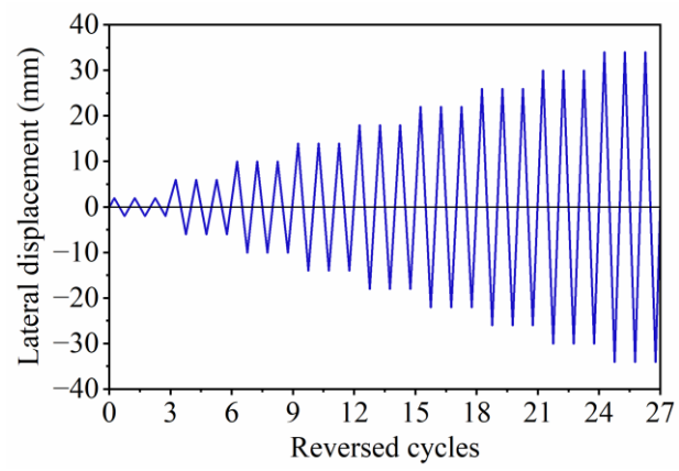
Fig. 1S. Loading protocol for reversed cyclic loading as per JGJ 2015
