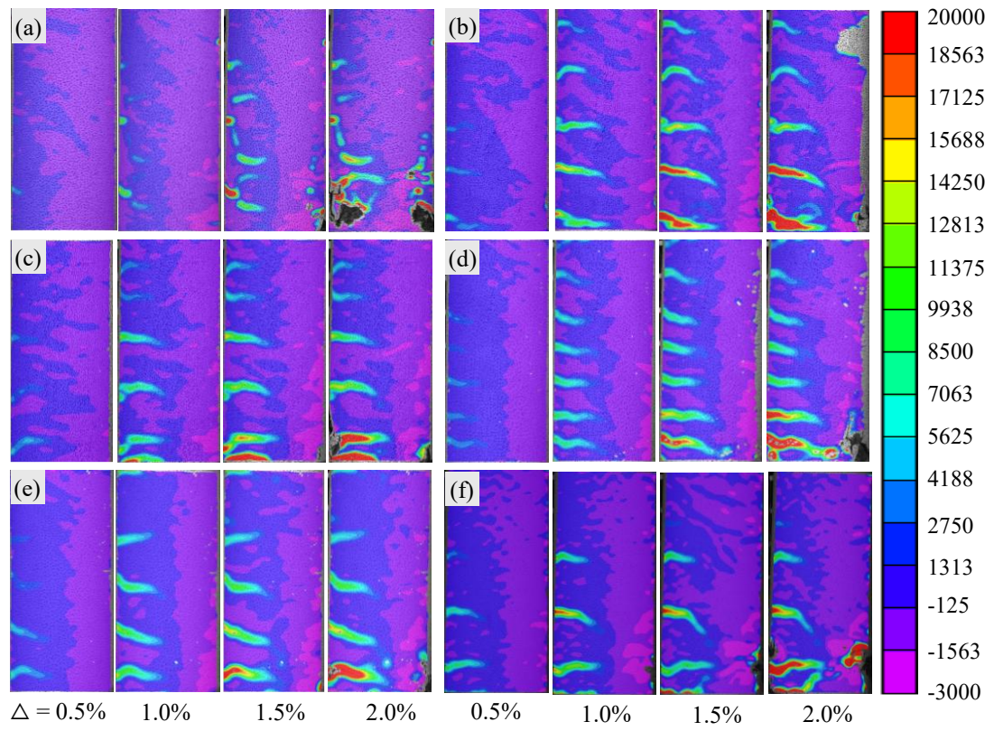
Fig. 3S. Strain ( e_{yy} ) evolution in push loading for: (a) SRC8Y-0; (b) HRC0N-0; (c) HRC8N-0; (d) HRC8Y-0; (e) HRC8Y-45; (f) HRC8Y-90
