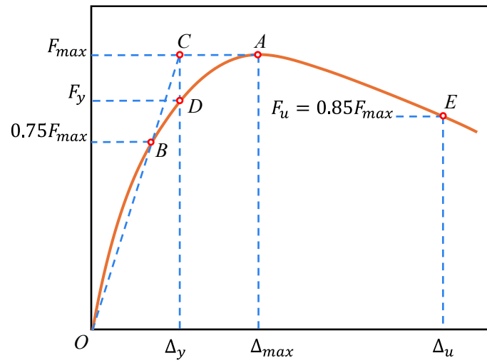
Fig. 6S. Schematic illustration of the Park method for yield point determination
