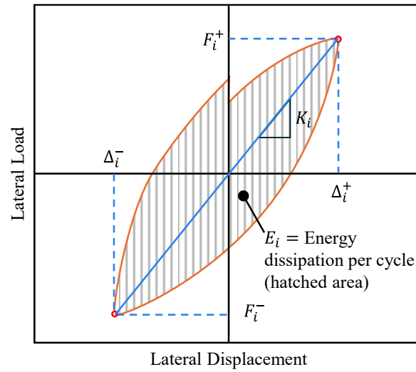
Fig. 7S. Schematic illustration of hysteresis-loop energy and stiffness calculation
