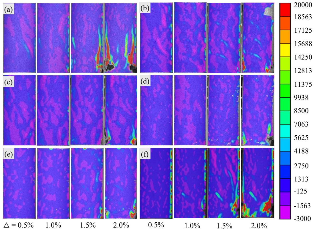
Fig. 4S. Strain ( e_{xx} ) evolution in push loading for: (a) SRC8Y-0; (b) HRC0N-0; (c) HRC8N-0; (d) HRC8Y-0; (e) HRC8Y-45; (f) HRC8Y-90
